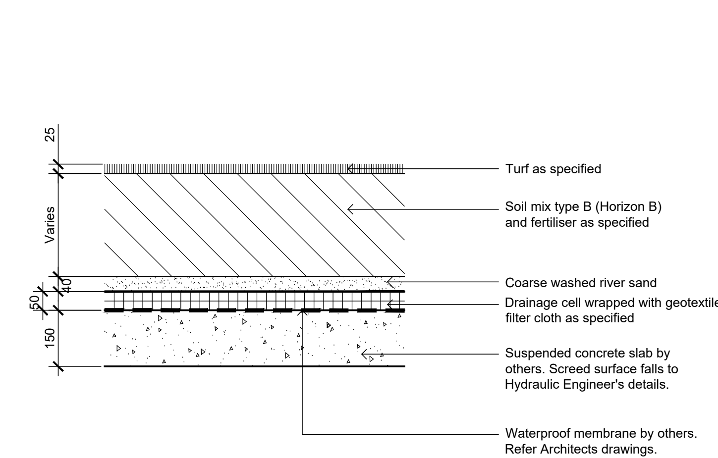
Detail Turf on Suspended Structure 1:10
